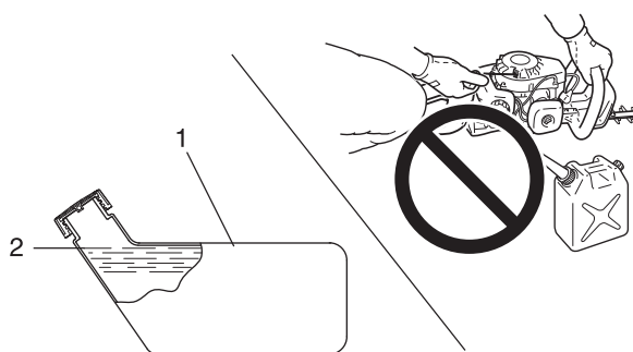
1. Brandstoftank
